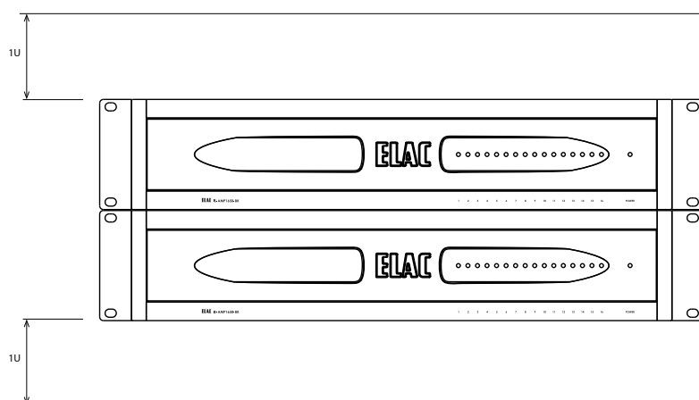
Figure 5 Spacing for amplifiers stacked mount
